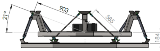
Figure 7: Home Position of the Platform Simulator
