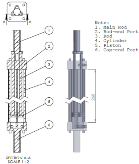
Figure 1: Multi Piston Pneumatic Actuator
