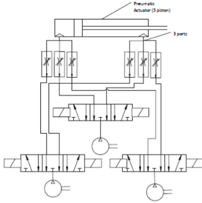
Figure 4: The Pneumatic Circuit Diagram
