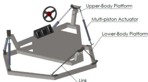
Figure 2: Three Dimension Platform Simulator
