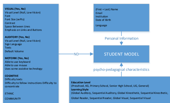
Fig. 1. Proposed Student Model
