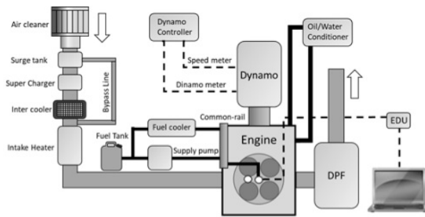
Fig. 1. Configuration of the experimental setup.
