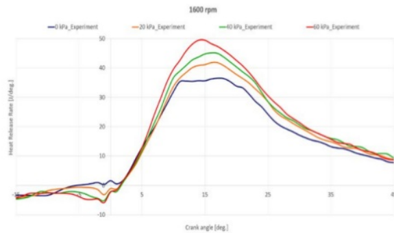
Fig. 3 Heat release rate with main injection timing of 1° ATDC for various boost pressures and engine rotation of 1600 RPM.
