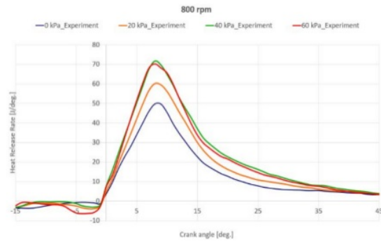
Fig. 1 Heat release rate with main injection timing of 1° ATDC for various boost pressures and engine rotation of 800 RPM.
