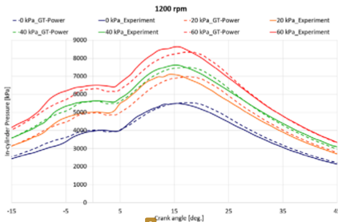
Fig. 4. 1-cylinder pressure with main injection timing of 1° ATDC for various boost pressures and engine rotation of 1200 RPM.
