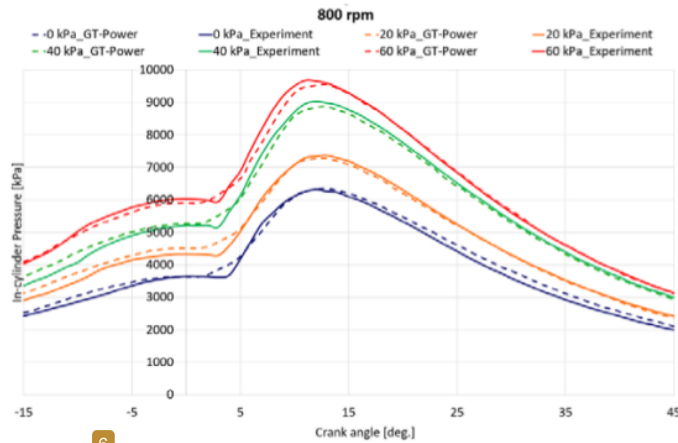
Fig. 3. 1-cylinder pressure with main injection timing of 1° ATDC for various boost pressures and engine rotation of 800 RPM.
