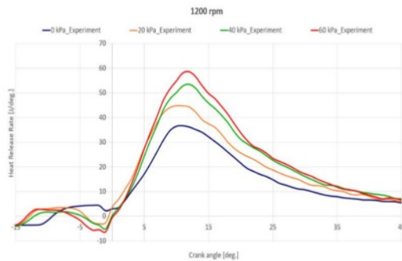
Fig. 2 Heat release rate with main injection timing of 1° ATDC for various boost pressures and engine rotation of 1200 RPM.
