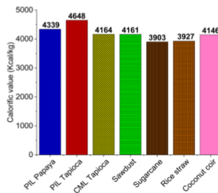
Figure 6. Comparison of various briquettes calorific value [13-15]. PIL is an abbreviation for Pterocarpus indicus leaves. CML is an abbreviation for Cerbera manghas leaves.
