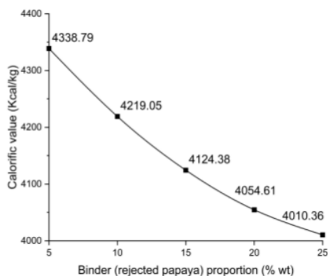
3 Figure 5. Calorific value of Pterocarpus indicus leaves waste and rejected papaya for various proportion (5% to 25%wt of rejected papaya).
