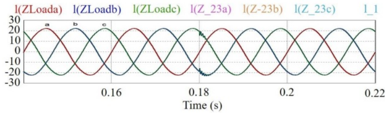
Figure 11 Load currents (= PCC currents = Transformer currents) after compensation
