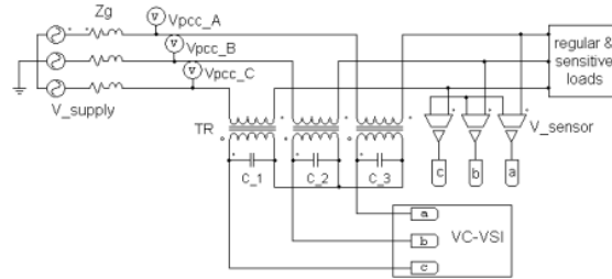
Figure 2 The position of the VC-VSI
