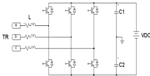
Figure 1 The three-phase four-wire VC-VSI power circuit
