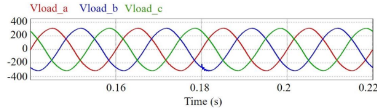
Figure 27 The load voltage after compensation for an unbalanced fault (SLGF) using the conventional compensator
