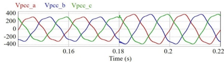
Figure 20 The PCC voltage under voltage rise
