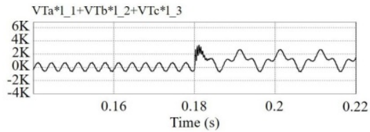
Figure 18 Active power from the VC-VSI for an unbalanced fault
