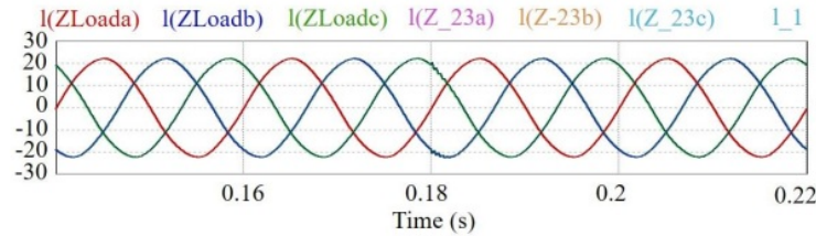
Figure 23 Load currents (= PCC currents = Transformer currents) after compensation
