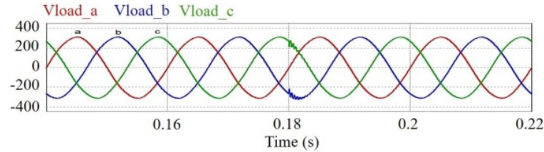
Figure 10 The load voltage after compensation for a balanced fault
