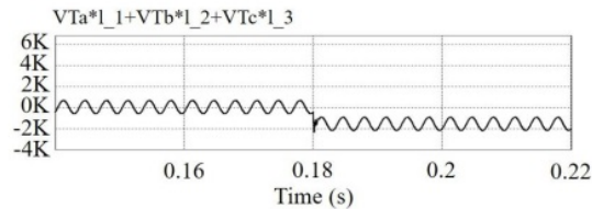
Figure 24 Active power from the VC-VSI for voltage rise
