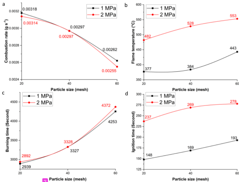
Figure 5. The combustion characteristics of Pterocarpus indicus leaves and rejected pineapple briquette. a) combustion rate, b) flame temperature, c) burning time, and d) ignition time
