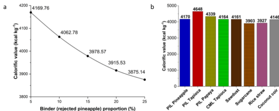
Figure 4. Comparison of a) the calorific value of briquettes for various proportions of biomass to binder, and b) the calorific value of briquettes for various biomasses and binders [7, 13, 19-21] with PIL is short for Pterocarpus indicus leaves and CML is short for Cerbera manghas leaves
