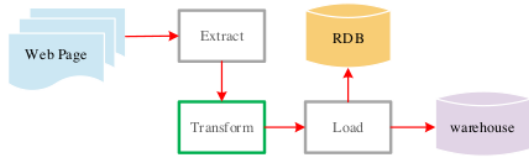
Fig. 4. ETL framework.
