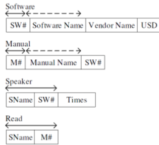
Fig. 7. Corresponding relational database schemas transformed from the ORM diagram in Fig. 6 based on the 2-step transformation.
