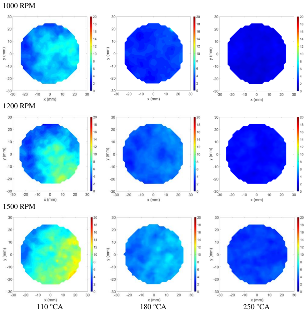
Figure 4 Turbulence intensity profile (in m/s) of the airflow under various engine speeds at 110, 180, and 250 CAD.
