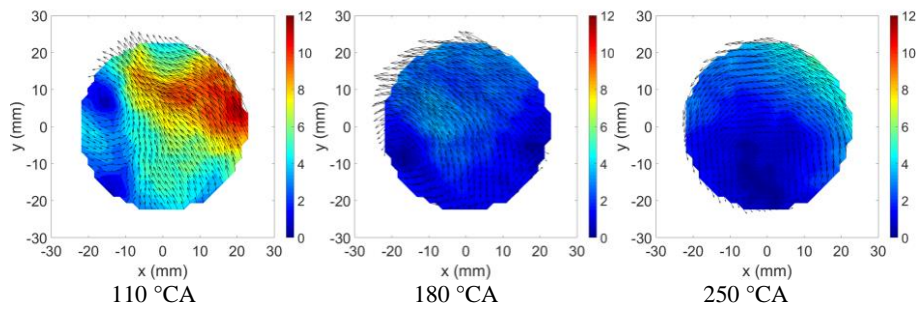
Figure 6 Mean velocity profile (in m/s) of the airflow under various SCV openings at 110, 180, and 250 CAD.
