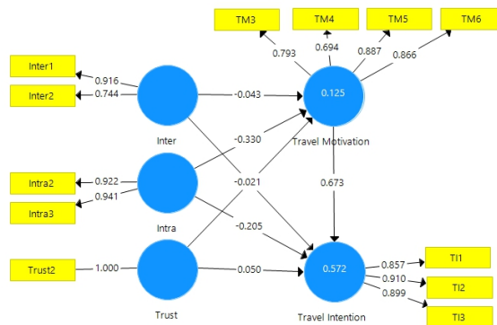
Fig 2. SEM Iteration phase 2 Model
