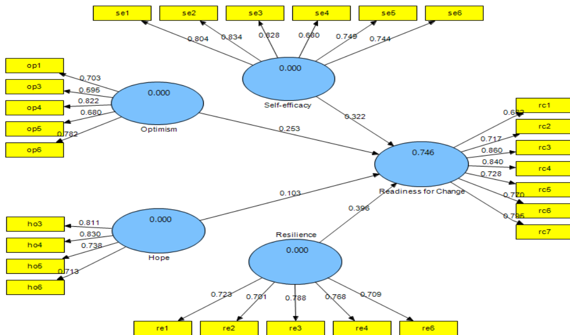
Figure 2. Path model and loading factor stage 2 (after dropping)
