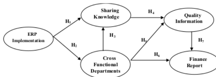
Fig. 1. Research framework
