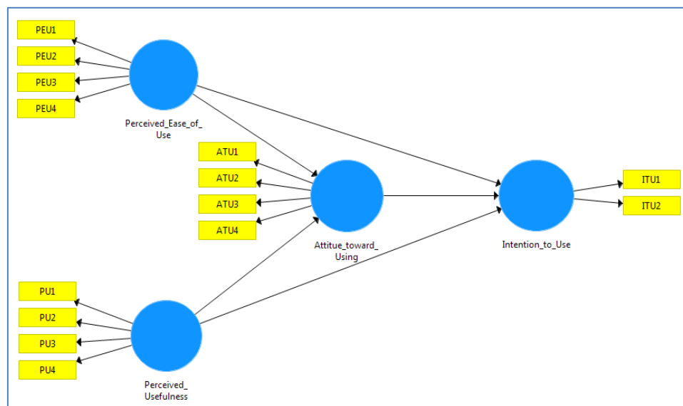
Figure 2 Path Diagram
