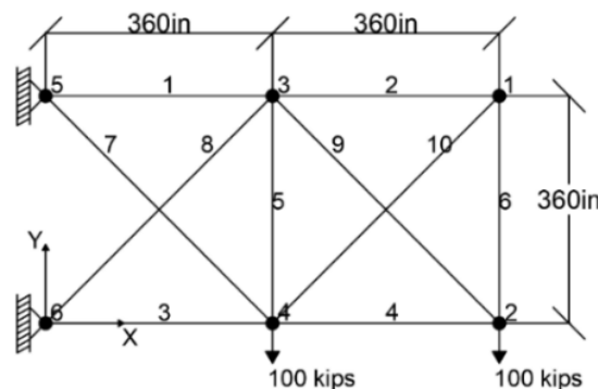
Figure 2. Ground structure for 10-bar truss structure.
