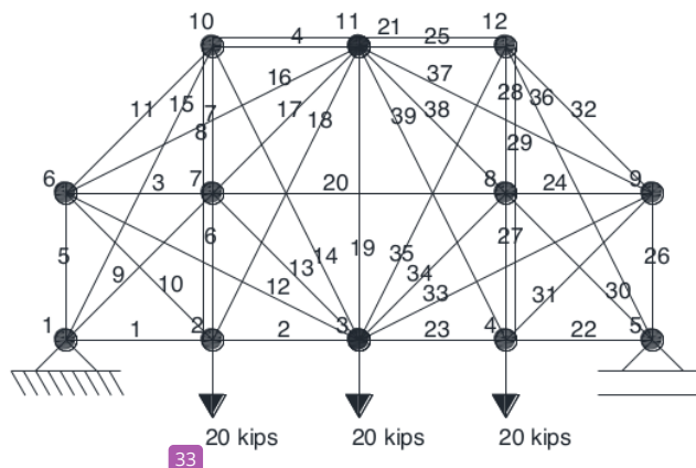
Figure 5. Ground structure for 39-bar truss structure.
