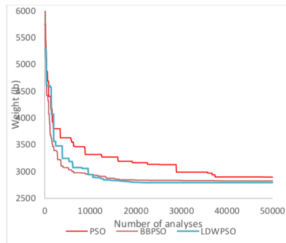
Figure 3. Convergence behavior for 10-bar truss structure.
