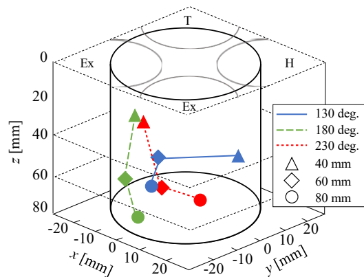
Fig. 8. Swirl centre position at each measurement plane.
