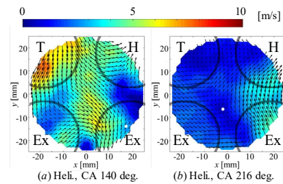
Fig. 11. Ensemble-averaged velocity-vector maps under 1000 rpm at Heli. during (a) CA 140 deg. and (b) CA 216 deg.
