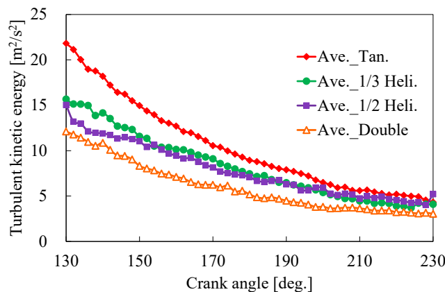
Fig. 16. Comparison of the time evolution of the in-cylinder average turbulent kinetic energy at different intake port opening ratios.
