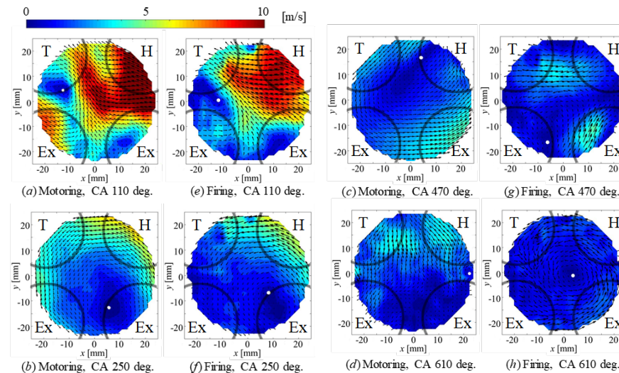
Fig. 2. Ensemble-averaged velocity-vector maps at z = 60 mm under motoring condition for (a) intake, (b) compression, (c) expansion and (d) exhaust stroke, and firing condition for (e) intake, (f) compression, (g) expansion and (h) exhaust stroke.
