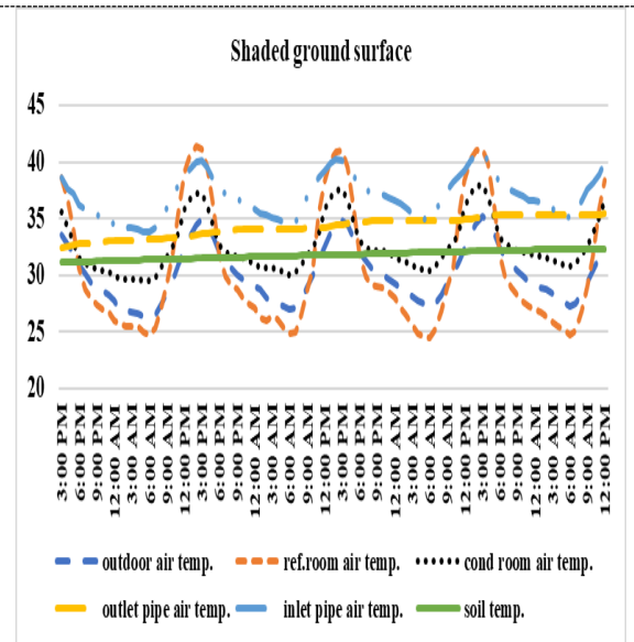
Figure 7. Hourly temperatures of outdoor air, referent room, condition room air, air in inlet pipe, air in outlet pipe and soil in shaded environment.
