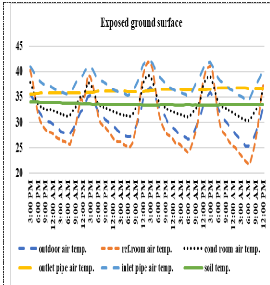
Figure 6. Hourly temperatures of outdoor air, referent room, condition room air, air in inlet pipe, air in outlet pipe and soil in exposed environment.
