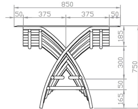
TAMPAK SAMPING
