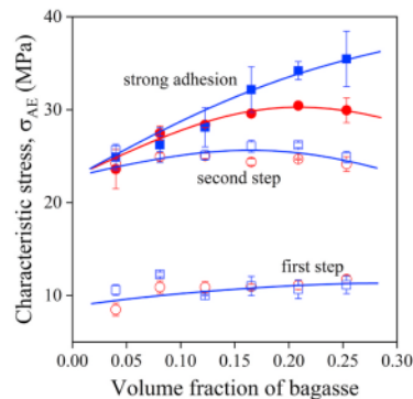
Fig. 7. Composition dependence of the characteristic (initiation) stresses of the local processes taking place around the fibers as determined by acoustic emission testing. Symbols: (x, ●) short fibers, (□, ■) long fibers; empty symbols: without MAPP, full symbols: with MAPP.
