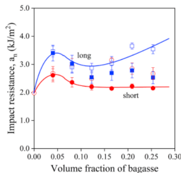
Fig. 4. Effect of fiber content on the notched Charpy impact resistance of PP/sugarcane bagasse fiber composites. Symbols: (x, ●) short fibers, (□, ■) long fibers; empty symbols: without MAPP, full symbols: with MAPP.
