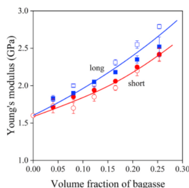
Fig. 2. Dependence of the stiffness of PP/sugarcane bagasse fiber composites on composition, initial fiber dimensions and interfacial adhesion. Symbols: (x, ●) short fibers, (□, ■) long fibers; empty symbols: without MAPP, full symbols: with MAPP.
