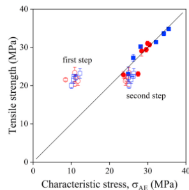
Fig. 8. Correlation between the tensile strength of the PP/bagasse fiber composites and the characteristic stresses of the local processes determined by acoustic emission testing. Symbols: (x, o) short fibers, (□, ■) long fibers; empty symbols: without MAPP, full symbols: with MAPP.
