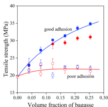
Fig. 3. Composition dependence of the tensile strength of PP/sugarcane bagasse fiber composites. Effect of interfacial adhesion. Symbols: (x, ●) short fibers, (□, ■) long fibers; empty symbols: without MAPP, full symbols: with MAPP.
