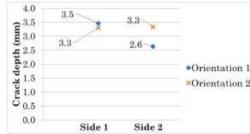
Figure 11. Gripper crack depth graph, orientations 1 and 2.
