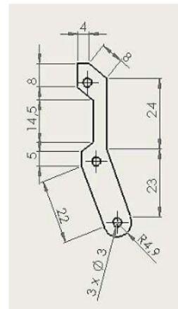
Figure 4. Gripper's dimension
