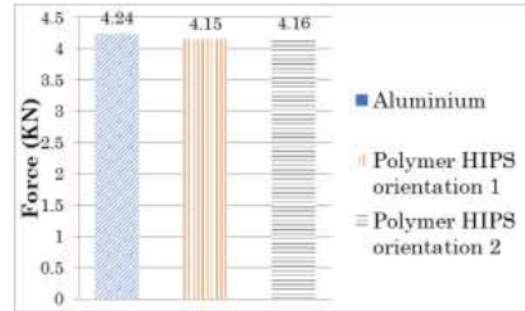
Figure 11. Flexural strength comparisons of grippers made of aluminium and polymer HIPS polymers (orientation 1 and 2)
