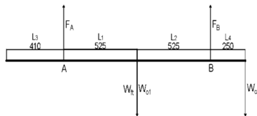
Figure 11. Free body diagram.
