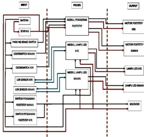
Figure 7. Schematic wiring diagram.
