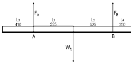
Figure 9. FBD of the footstep.
