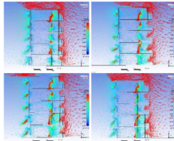
Fig 19. Wind movement in model 5-8 at wind angle 45° (Source: Author, 2022)
