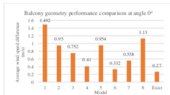
Fig 14. Overall performance of all models at angle 0° (Source: Author, 2022)
