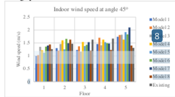
Fig 9. Max indoor wind speed at angle 45° (Source: Author, 2022)
