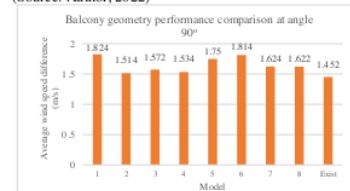
Fig 8. Overall performance of all models at angle 90° (Source: Author, 2022)
