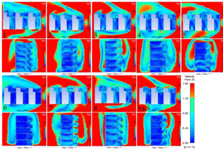
Fig 20. Plane visuals of wind distribution and penetration on floor 3 at angle 0° (Source: Author, 2022)
