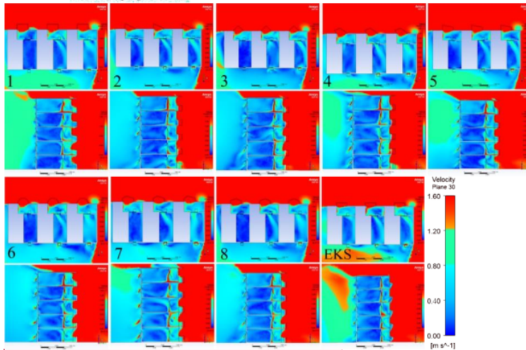
Fig 18. Plane visuals of wind distribution and penetration on floor 3 at angle 45° (Source: Author, 2022)
