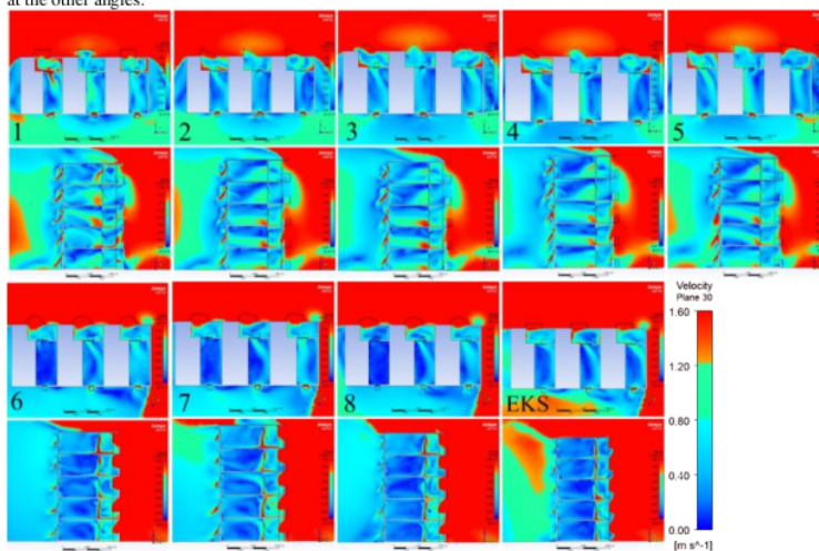
Fig 16. Plane visuals of wind distribution and penetration on floor 3 at angle 90° (Source: Author, 2022)
