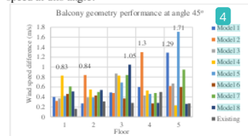
Fig 10. Balcony geometries performance at angle 45° (Source: Author, 2022)
