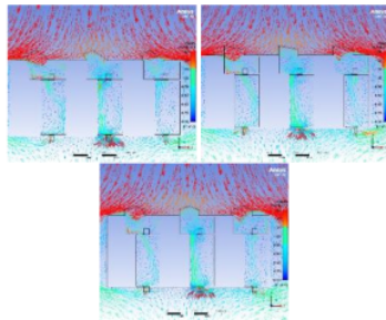
Fig 17. Wind movement on model 4, 5, 8 plans at angle 90° (Source: Author, 2022)
