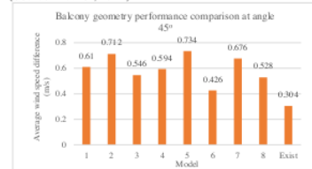
Fig 11. Overall performance of all models at angle 45° (Source: Author, 2022)
