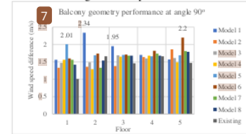
Fig 7. Balcony geometries performance at angle 90° (Source: Author, 2022)
