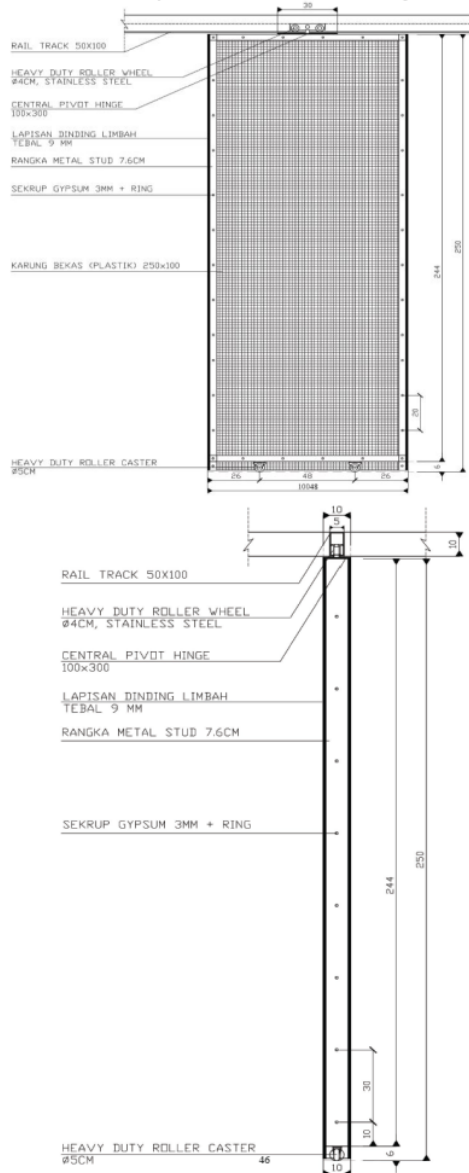
Fig. 10. Details of adaptive wall
