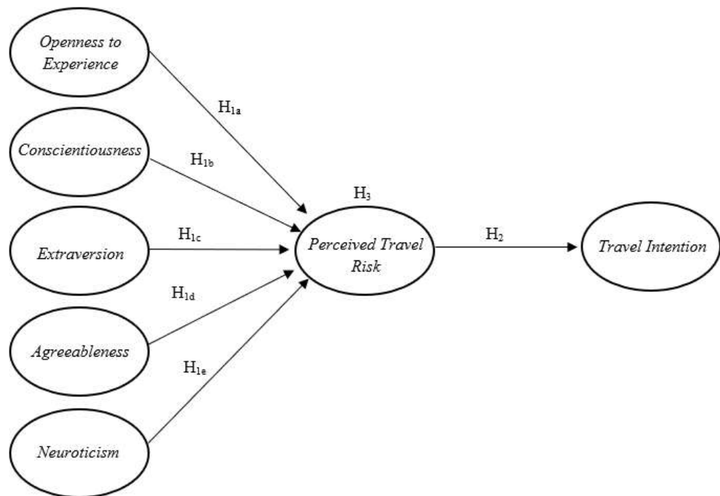
Figure 1. Research Model
