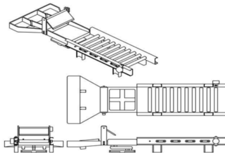
Gambar 4. Proses Instalasi Belt dan Roller Conveyor
