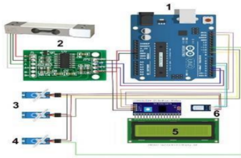
Gambar 5. Wiring Diagram Sistem Separator
