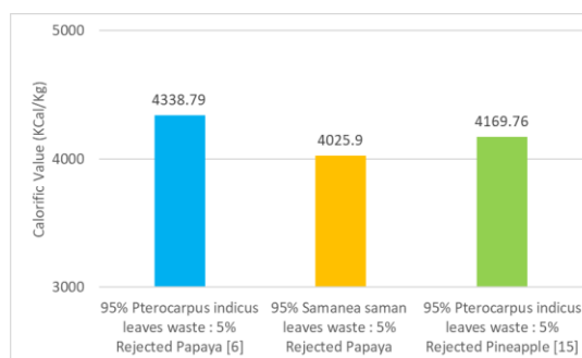
Figure 7. Calorific value of various briquettes
