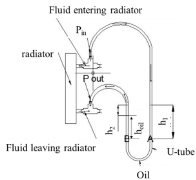
(b) Location of U-tube
