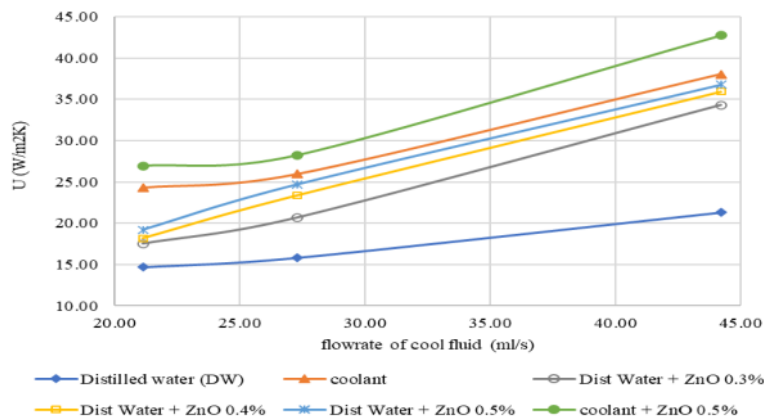
16 FIGURE 7. The overall heat transfer coefficient in the radiator.
