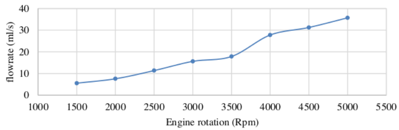
FIGURE 3. The cooling fluid flow rate at a different engine rotation speed
