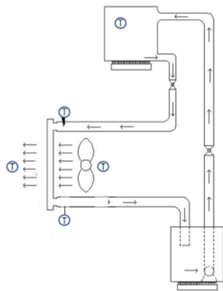
(a) Location of K-type thermocouple
