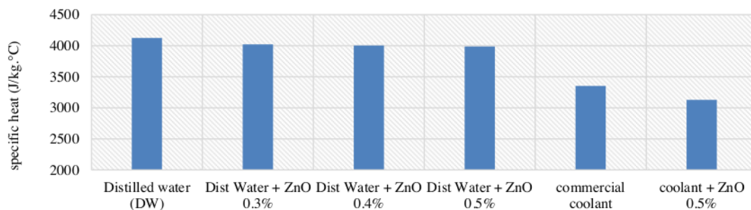
FIGURE 2. The specific heat of six fluids in this study
