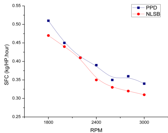
Figure 5. SFC engine test results of various diesel fuels with respond to RPM changes.
