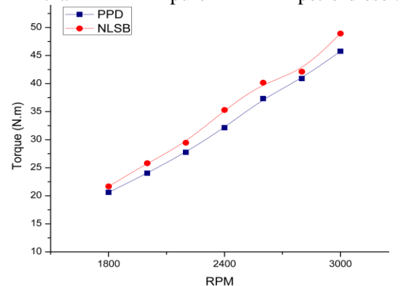
Figure 3. Torque engine test results of various diesel fuels with respond to RPM changes.
