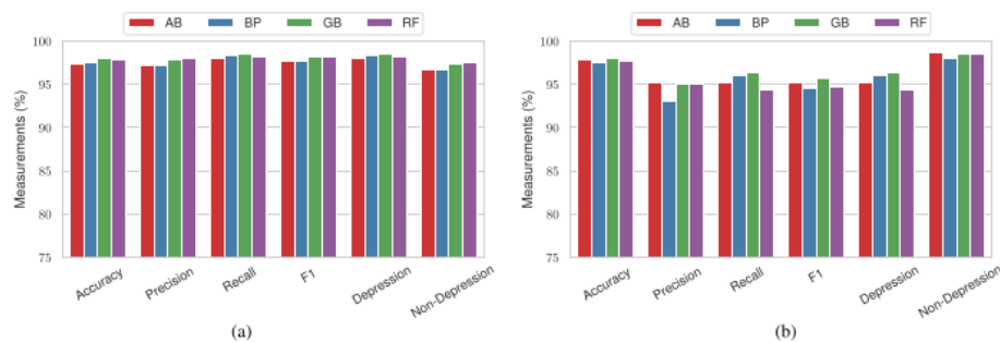
FIGURE 3. Results for feature groups A-G on ensemble models trained using two different datasets.
