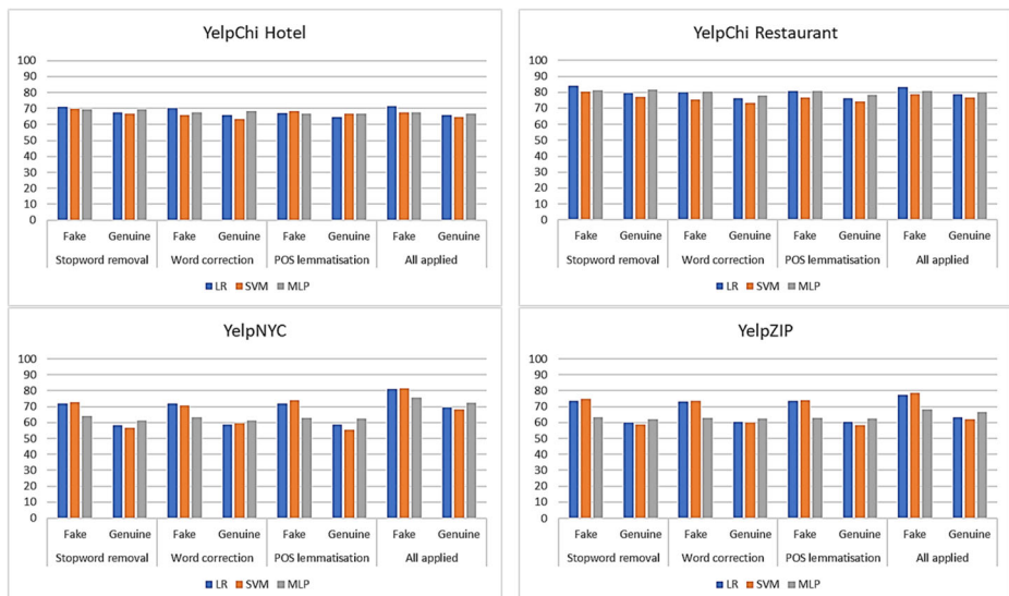
Fig. 5 Accuracy of each preprocessing step for under-sampling prediction (in percentage)
