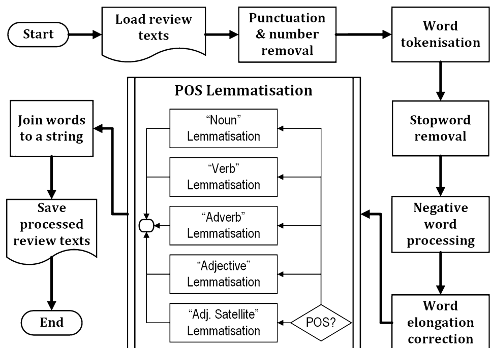
Fig. 7 Pre-processing steps with negation words, word elongation, and POS lemmatisation
