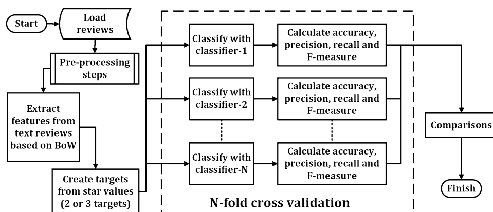
Fig. 1 A comparison framework for rating polarity
