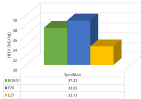
Gambar 2. Perbandingan nilai High Heating Value
