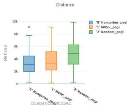
Fig. 3. Boxplot Distance
