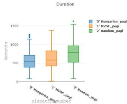
Fig. 2. Boxplot Duration
