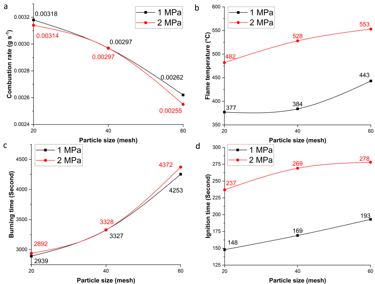
Figure 5. The combustion characteristics of Pterocarpus indicus leaves and rejected pineapple briquette. a) combustion rate, b) flame temperature, c) burning time, and d) ignition time
