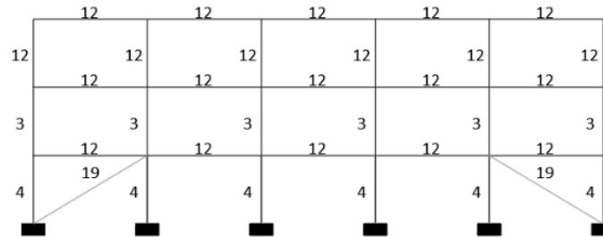
Figure 4. Lightest structure for a three-story concentrically braced frame with section numbers based on Tables 4 and 5
