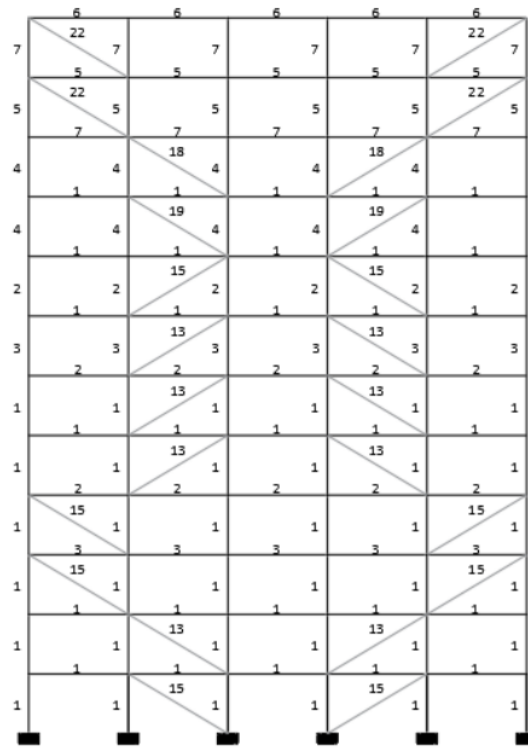
Figure 10. Lightest structure for a twelve-story concentrically braced frame with section numbers based on Tables 4 and 5
