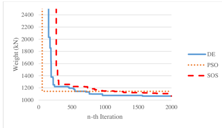
Figure 9. Convergence graph median result for a twelve-story frame
