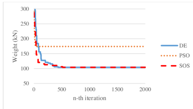
Figure 3. Convergence graph median results for a three-story frame
