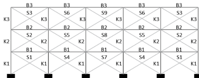
Figure 2. Column, beam, and bracing grouping variable for three-story frame
