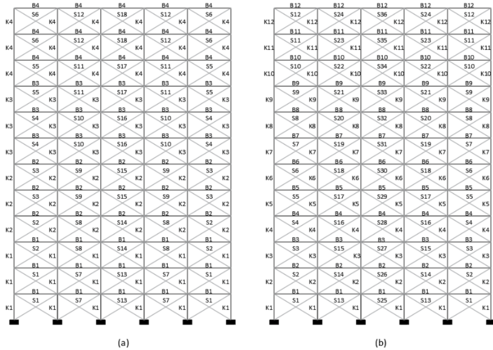
Figure 8. Column, beam, and bracing grouping variable for the first phase (a) and second phase (b) of a twelve-story frame
