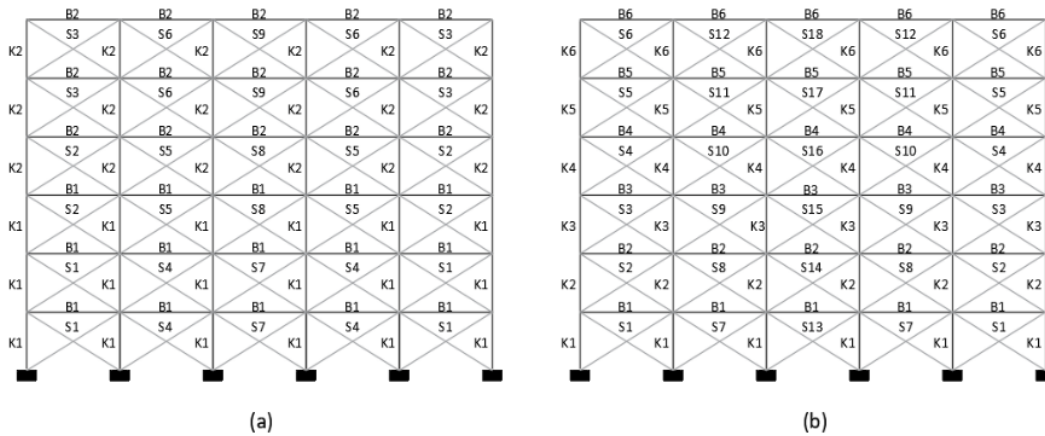
Figure 5. Column, beam, and bracing grouping variable for the first phase (a) and second phase (b) of a six-story frame
