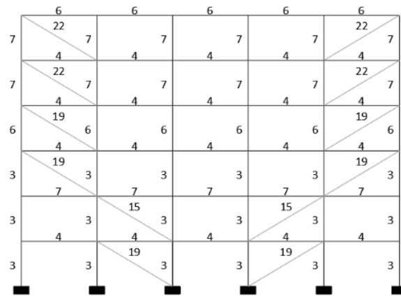
Figure 7. Lightest structure for six-story concentrically braced frame with section numbers based on Tables 4 and 5
