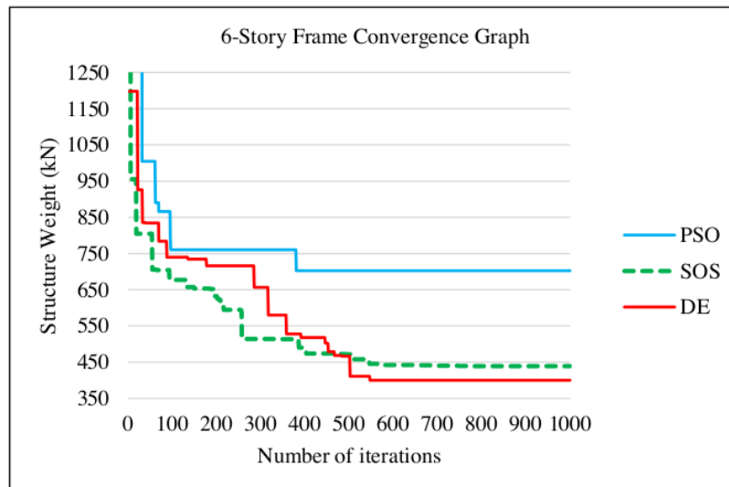
Figure 4. 6-story frame convergence graph
