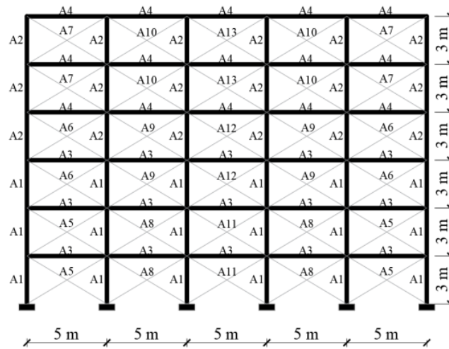
Figure 2. Front view of a 5-span, 6-story frame structure.
