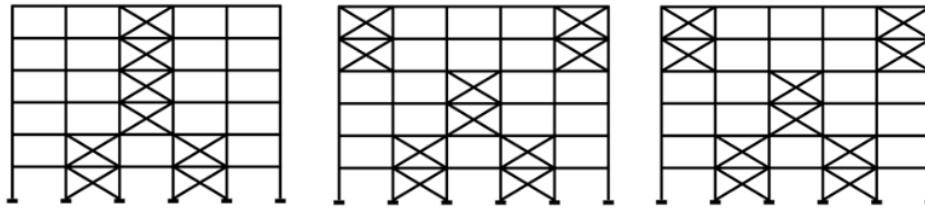
Figure 3. Brace placement of the 5-span, 6-story concentrically braced steel frame structure.
