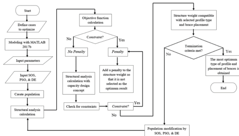
Figure 1. Research Flowchart.
