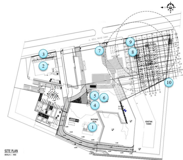
Fig. 1. Construction site layout plan for the employed project.
