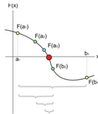
Fig. 4. Bisection Method
