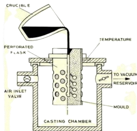
Gambar 1. Prinsip Vacuum Casting
