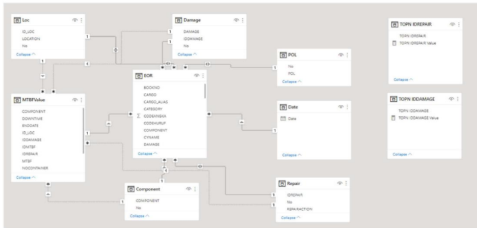
Figure 1. Data relationship diagram
