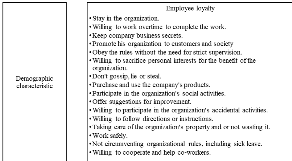
Fig. 1. Research Framework.
