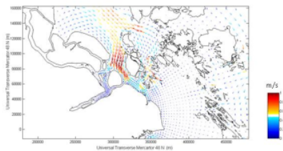
Figure 4: Current magnitude during spring-ebb flow for the regional model at Galang Island
