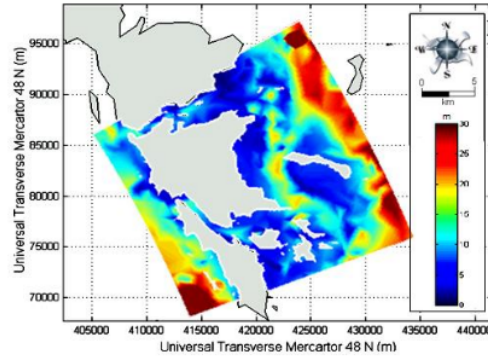
Figure 3: Galang Island-Local Model bathymetry
