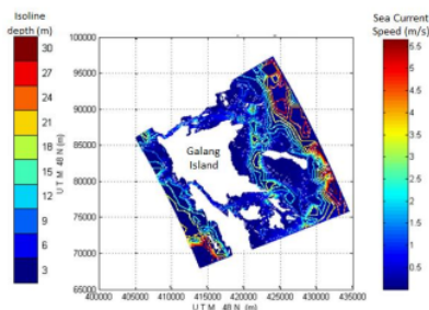
Figure 6: Predicted Maximum Sea Current Velocities in the vicinity of Galang Island using Delft3D Software and Grid Spacing of 44 m to 52 m
