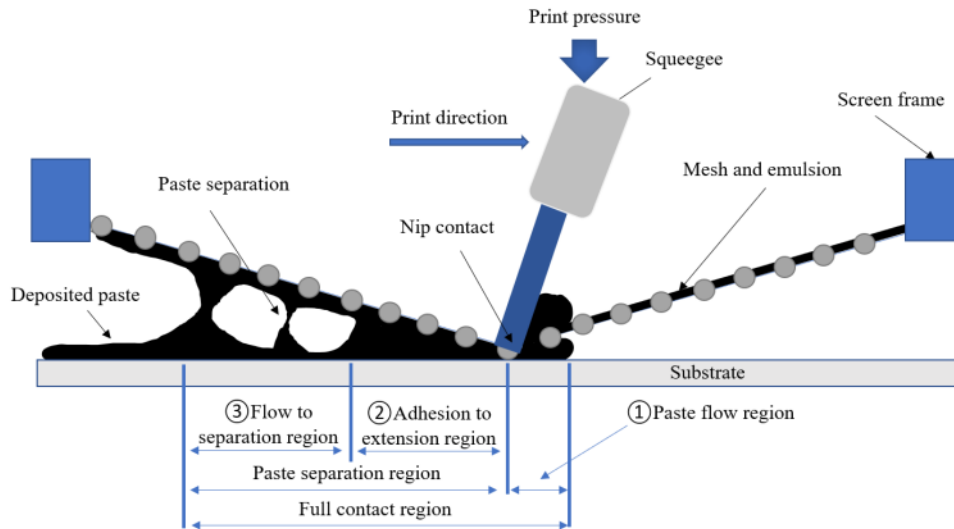
Fig. 2 Illustration of the screen-printing process
