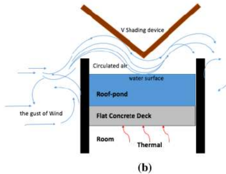
Figure 6. (a) Wind breezes pattern over common roof-pond (b) Laminar wind breezes behavior with V shape shading devices.
