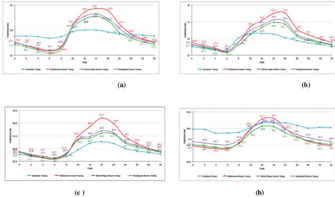
Figure 10. (a) Hourly Average Room Ambient Temperatures March 2021, (b) Hourly Average Room Ambient Temperatures June 2021, (c) Hourly Average Room Ambient Temperatures September 2021, (d) Hourly Average Room Ambient Temperatures December 2021.
