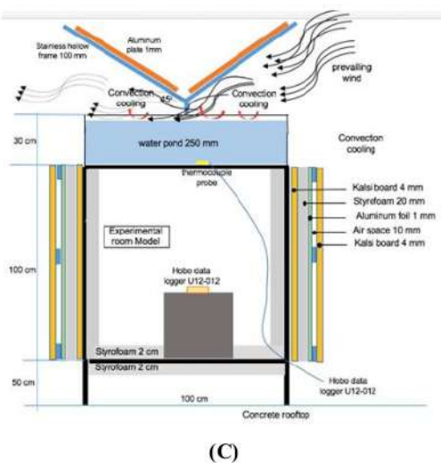
Figure 3. (a) Conventional concrete rooftop with V shading device, (b) Conventional roof-pond with V shading device, and (c) Wind-driven roof-pond with submerged iron tubes and V shape shading devices.
