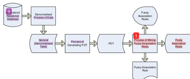
3 Fig. 1. Process of Mining Association Rules
