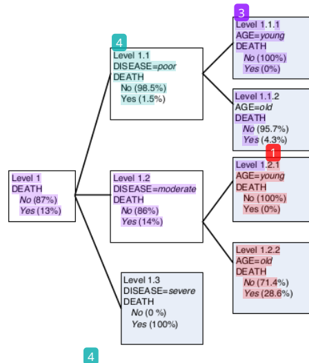
Fig. 7. The Generated Decision Tree
