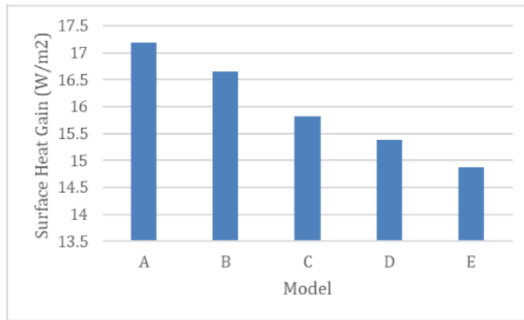
Figure 5. Solar incident radiation on second skin façade
