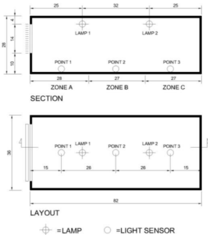
Figure 6: Layout plan and section of the model
