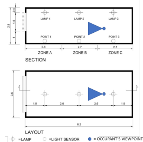
Figure 10: Layout plan and section of the model built in Rhino/Grasshopper simulation software.
