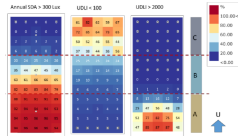
Figure 3: Annual SDA and UDI simulation results.
