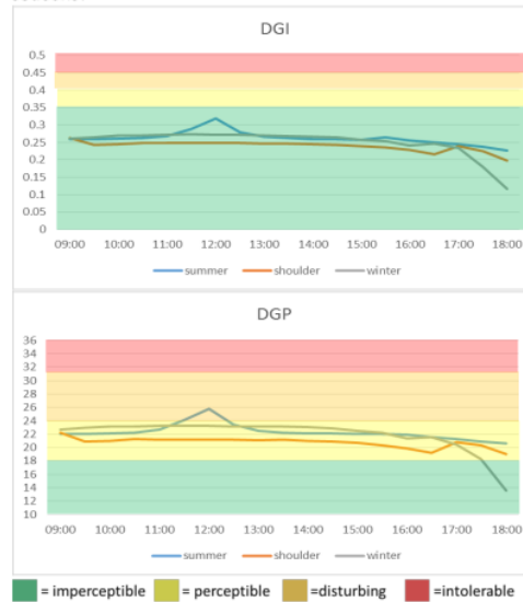
Figure 13: Glare analysis during the shoulder, summer, and winter seasons.
