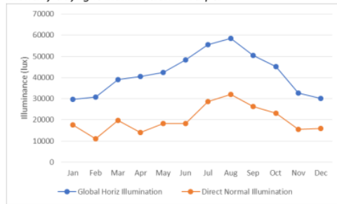
Figure 1: Monthly daylight illumination in Taipei
