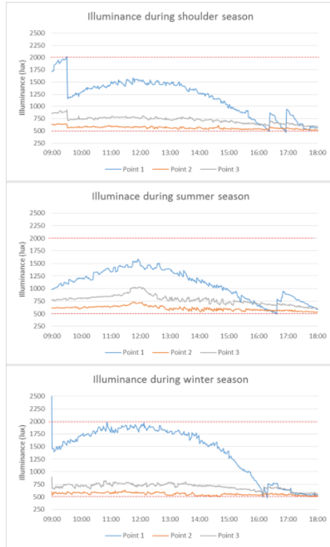
Figure 11: Indoor illuminance values during the shoulder, summer, and winter seasons.
