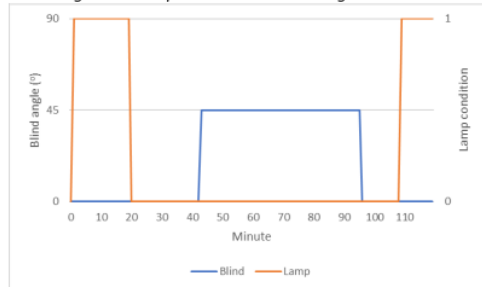
Figure 9: Blind angle and lamp condition monitoring.
