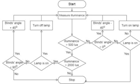
Figure 4: Algorithm flow of the control strategies.
