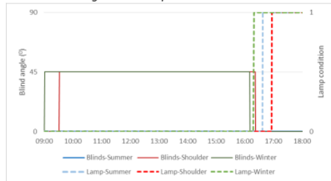
Figure 12: Annual blind angles and lamp 1 condition.
