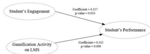
Fig. 2. Regression Model
