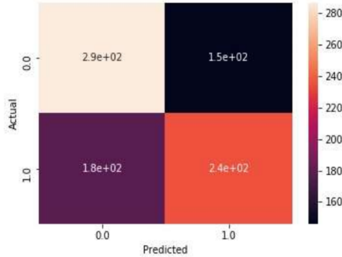
FIGURE 3. Confusion matrix of random forest next-day-prediction
