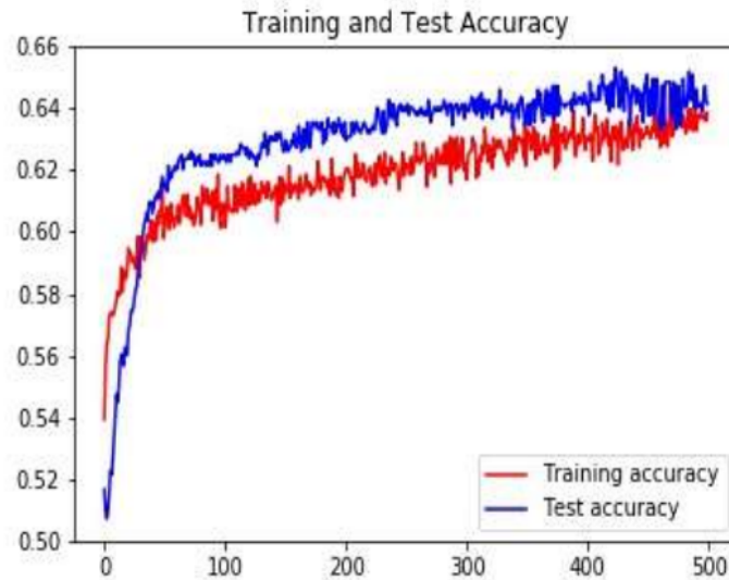
FIGURE 4. Training and testing accuracy
