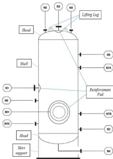
FIGURE 1. Design Concept of Two-Phase Scrubber
