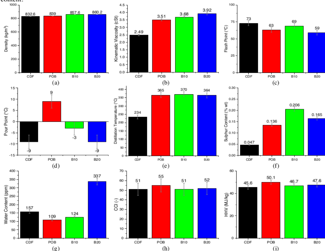
FIGURE 1. Results of the fuel property tests for (a) density, (b) kinematic viscosity, (c) flash point, (d) pour point, (e) distillation temperature, (f) Sulphur content, (g) water content, (h) CCI (calculated cetane index), and (i) HHV (higher heating value). CDF and POB are abbreviation of the conventional diesel fuel and palm oil biodiesel, respectively. The error bars for density results are not clearly visible since the uncertainty of the measurements is small.
