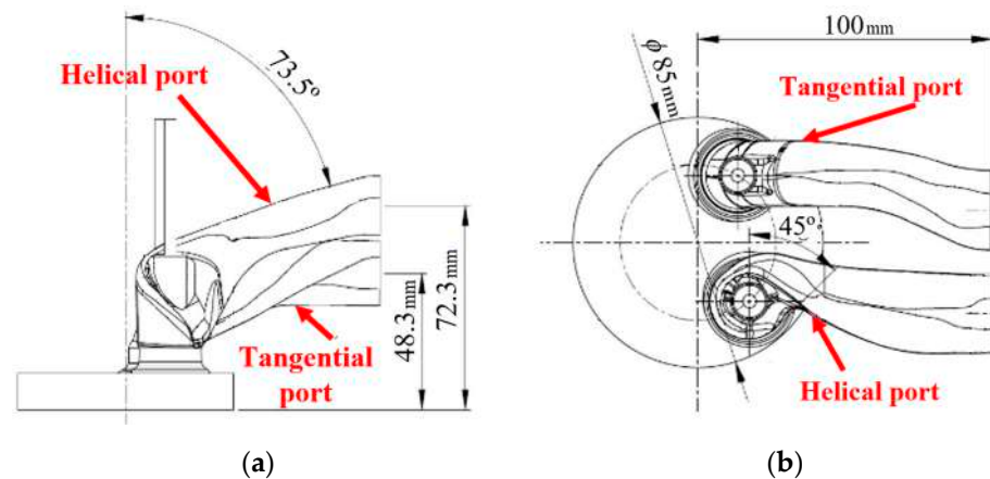
Figure 2. (a) Side view and (b) top view of the helical and tangential intake ports.
